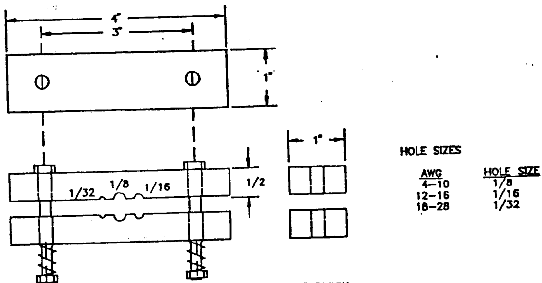
FIG. 3 CIRCUMFERENTIAL ELONGATION SPECIMEN HOLDING BLOCK
