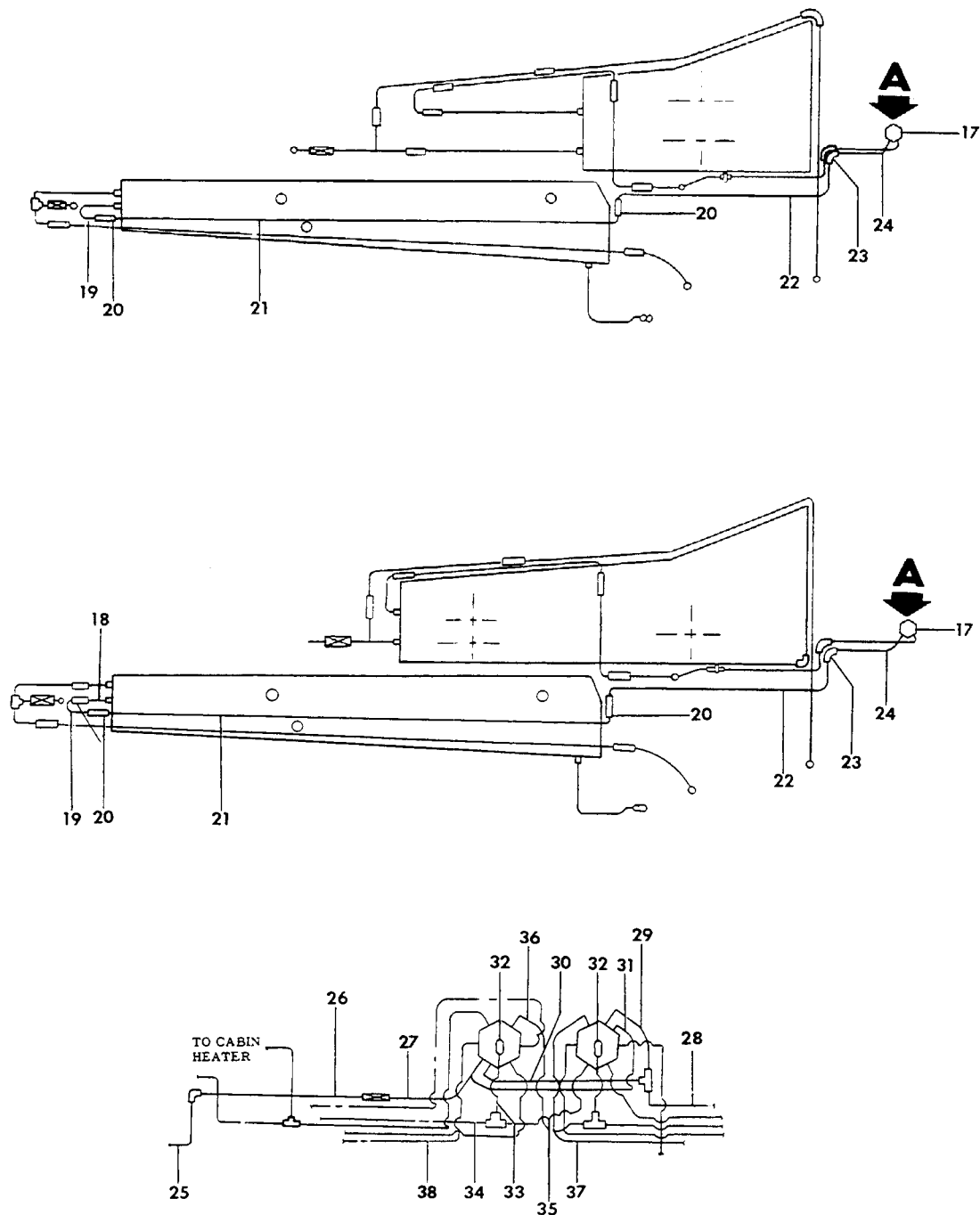
VIEW A
