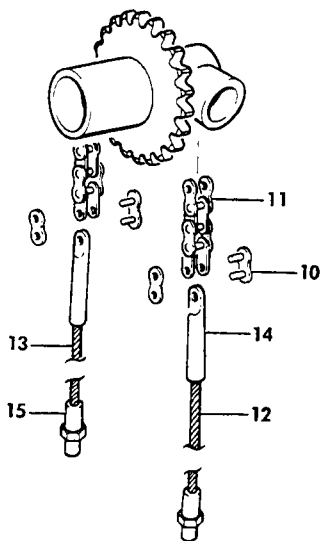
VIEW B
