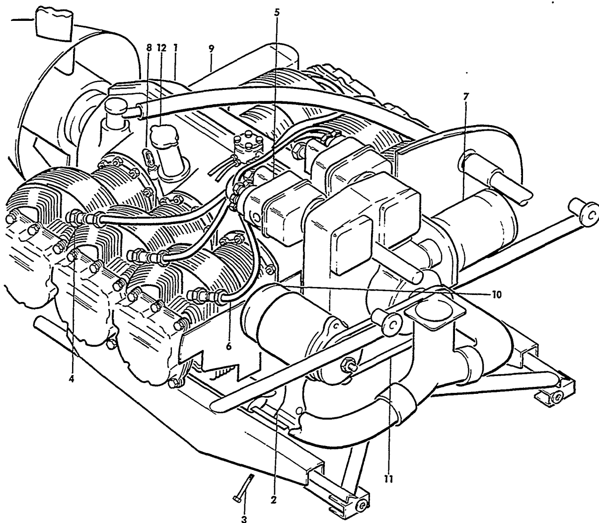
VIEW A
