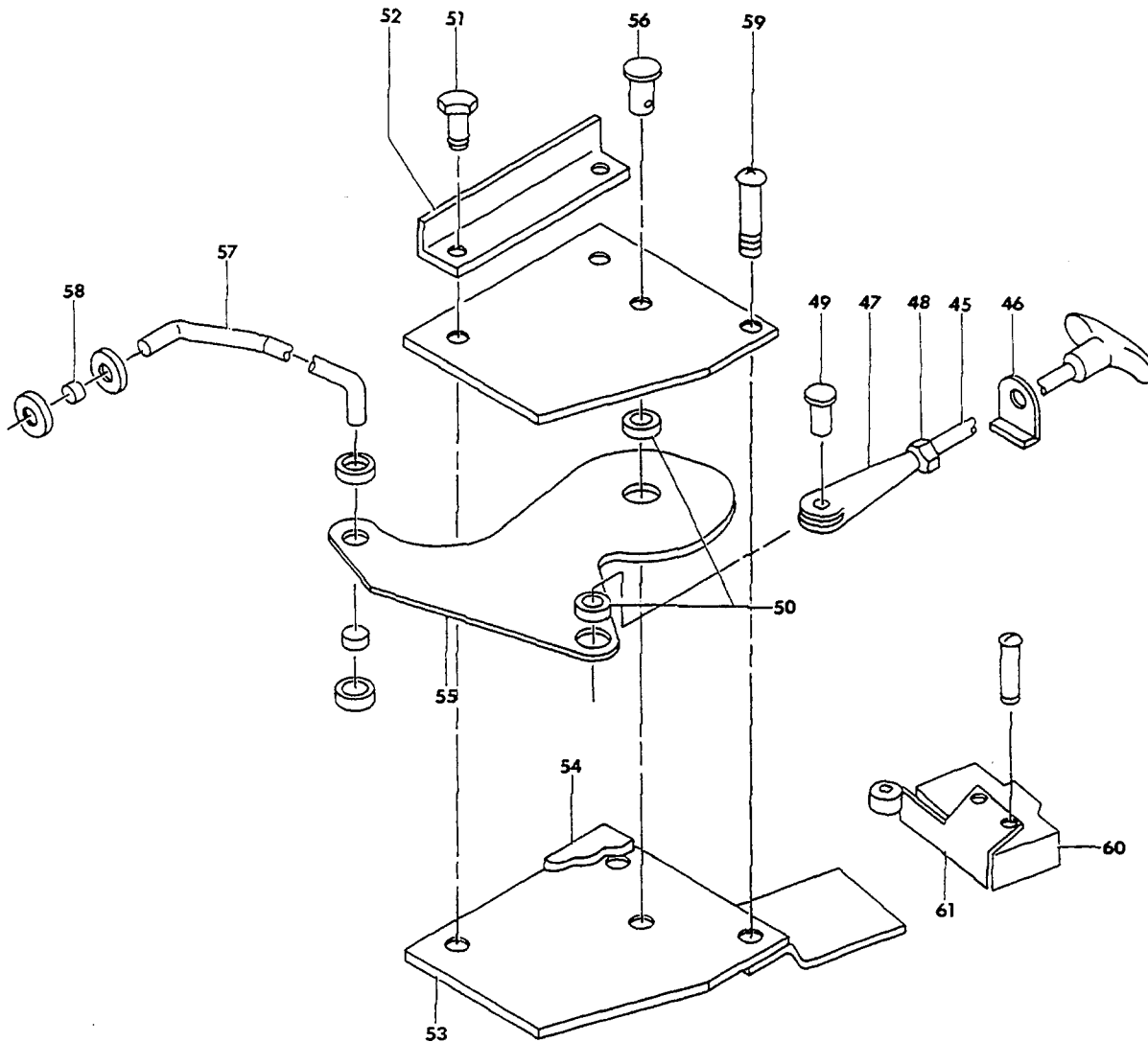
VIEW B
