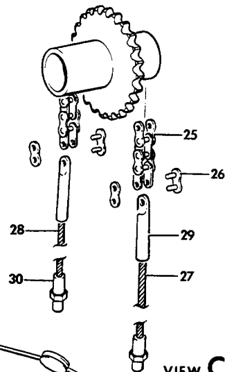
VIEW C
