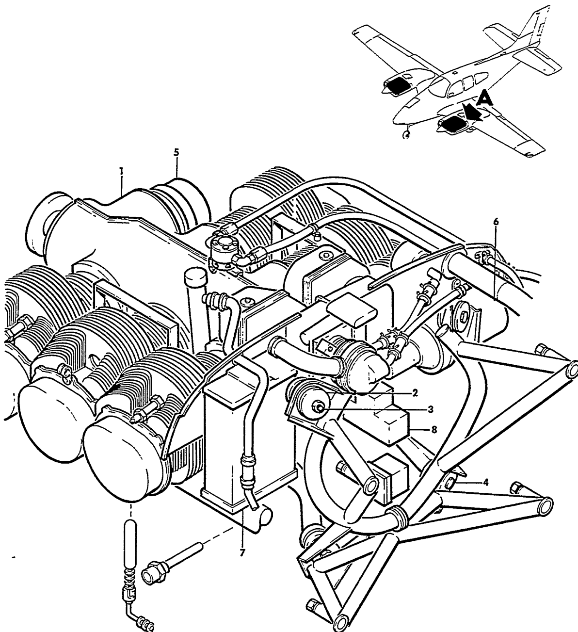
VIEW A
