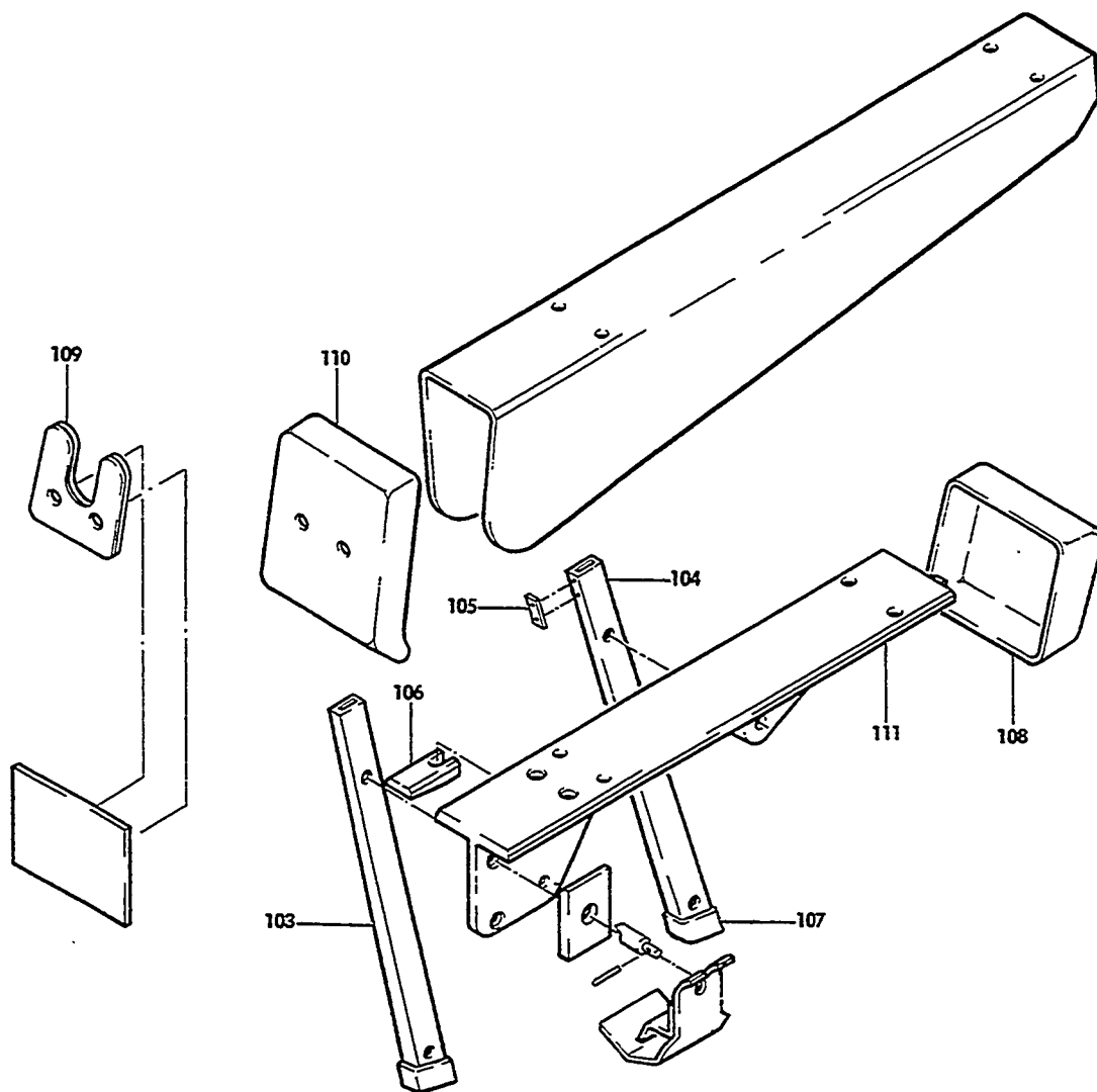
VIEW A
