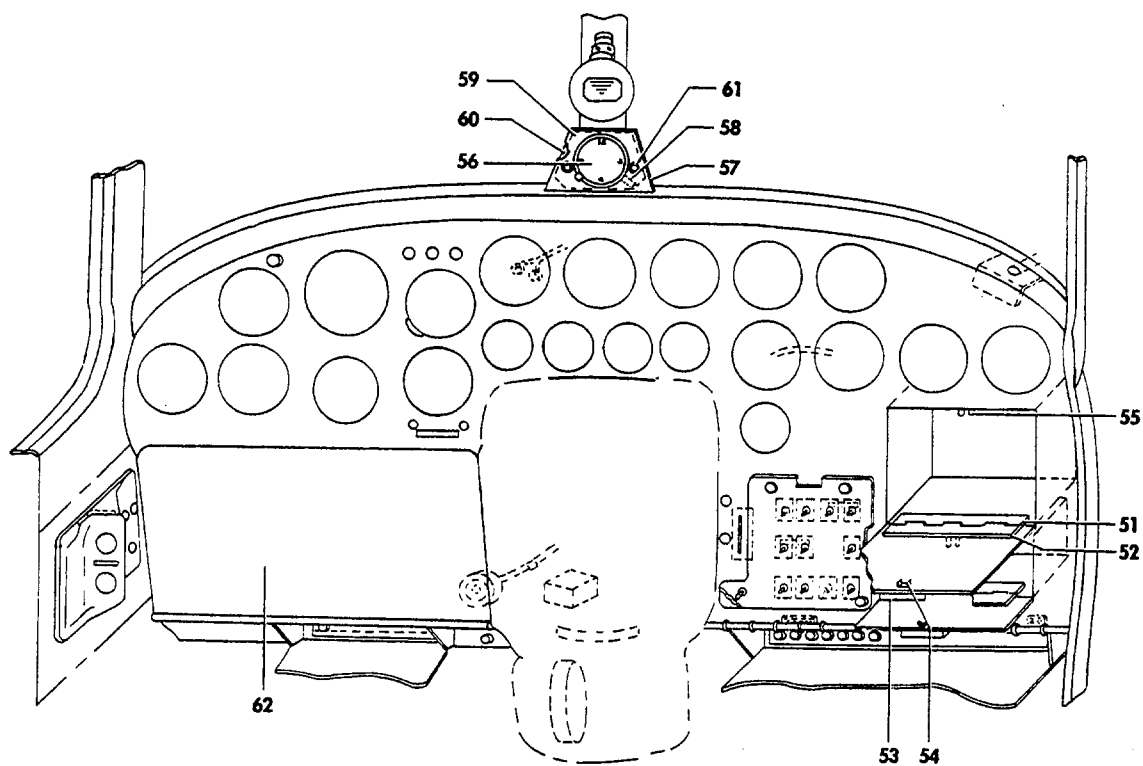
VIEW A
