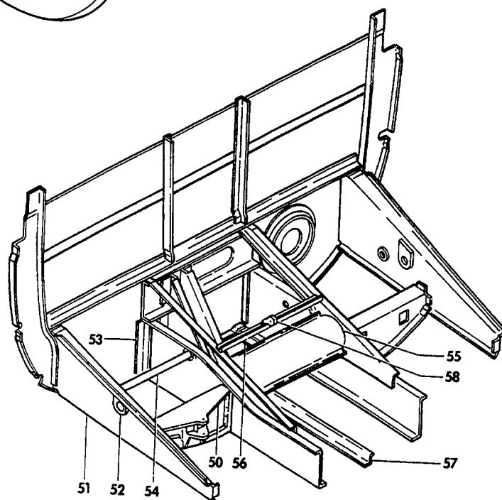
VIEW A
