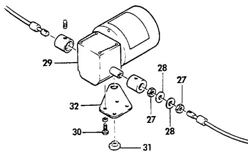
VIEW A
