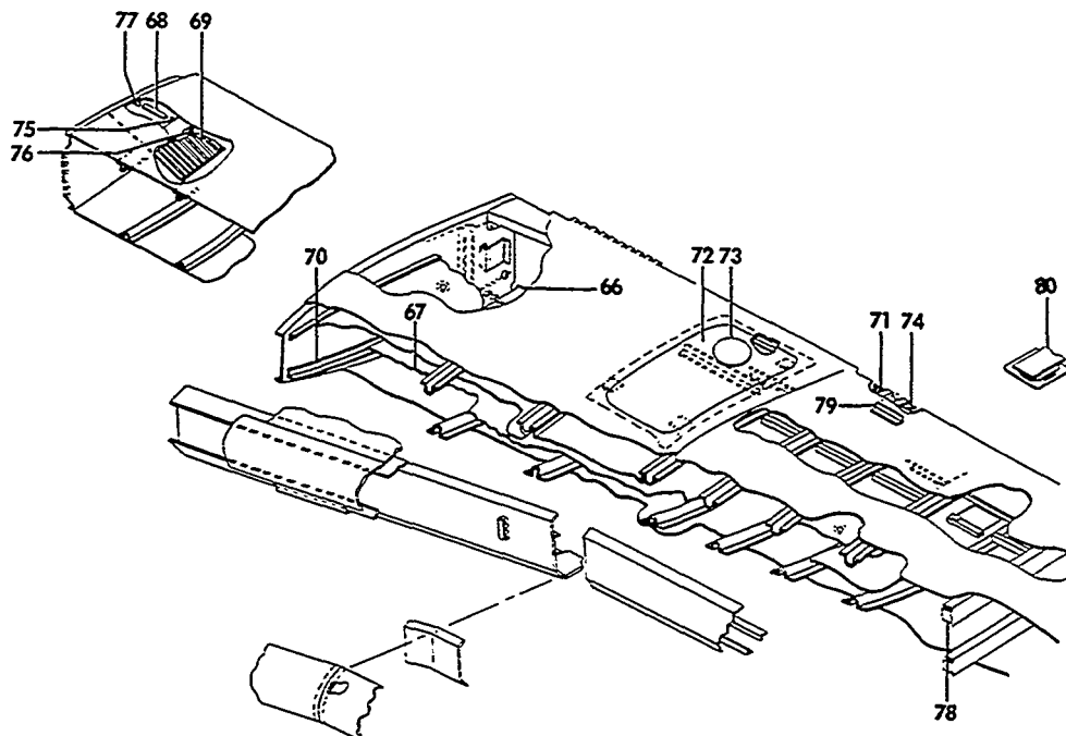
VIEW A
