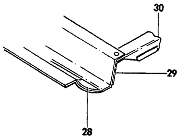
VIEW A
