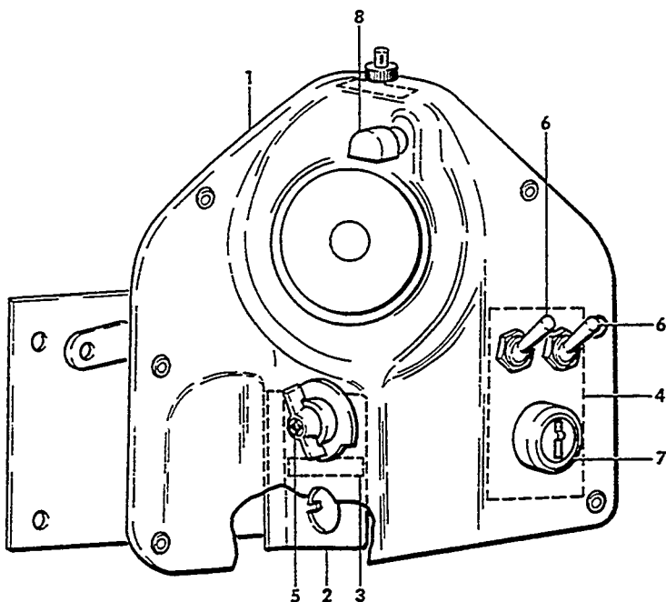
VIEW A
