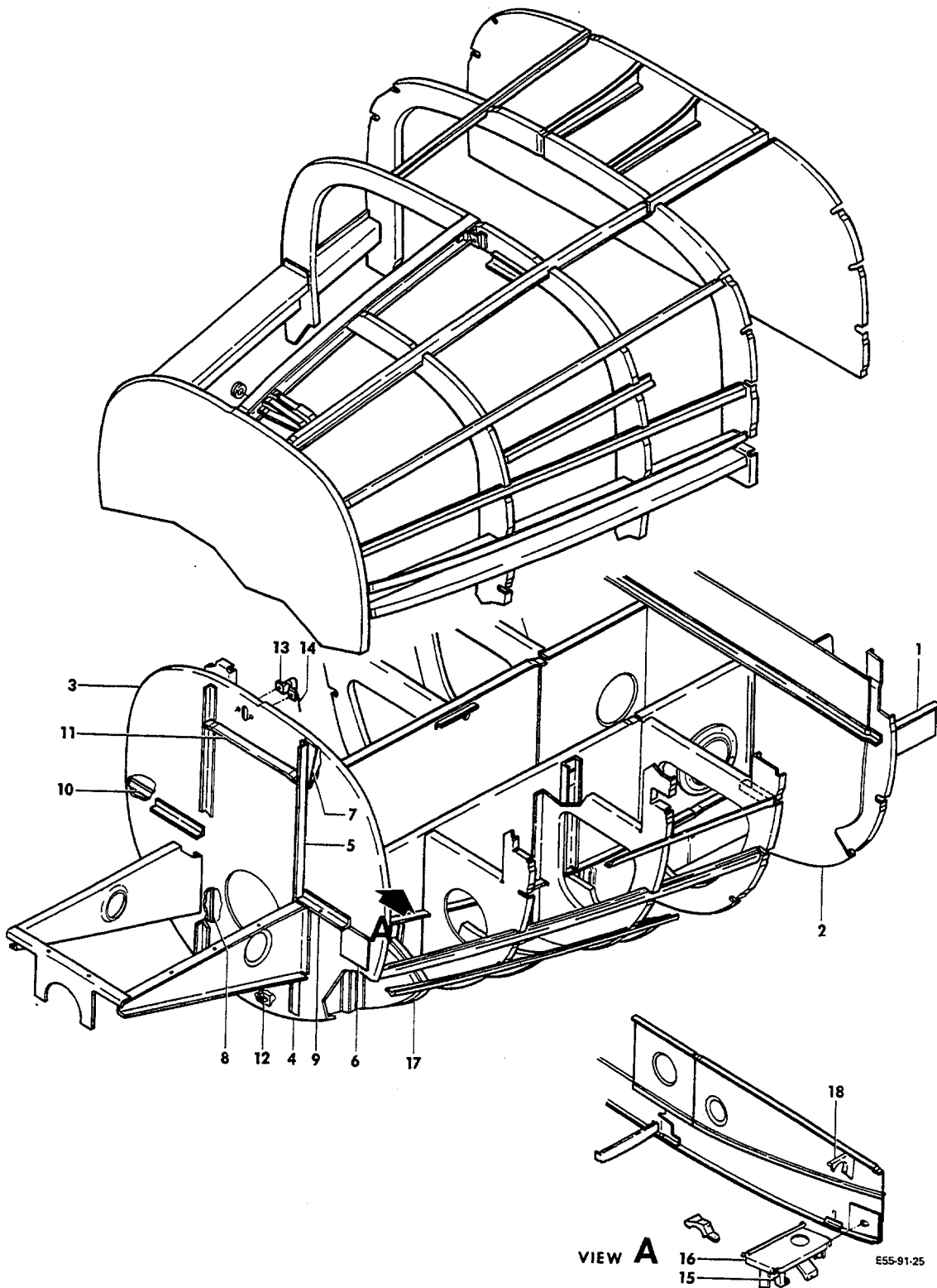
FIGURE 11-C1.NOSE STRUCTURE /SHEET 1 OF 5 SHEETS/
