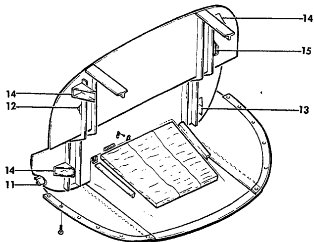
VIEW A
