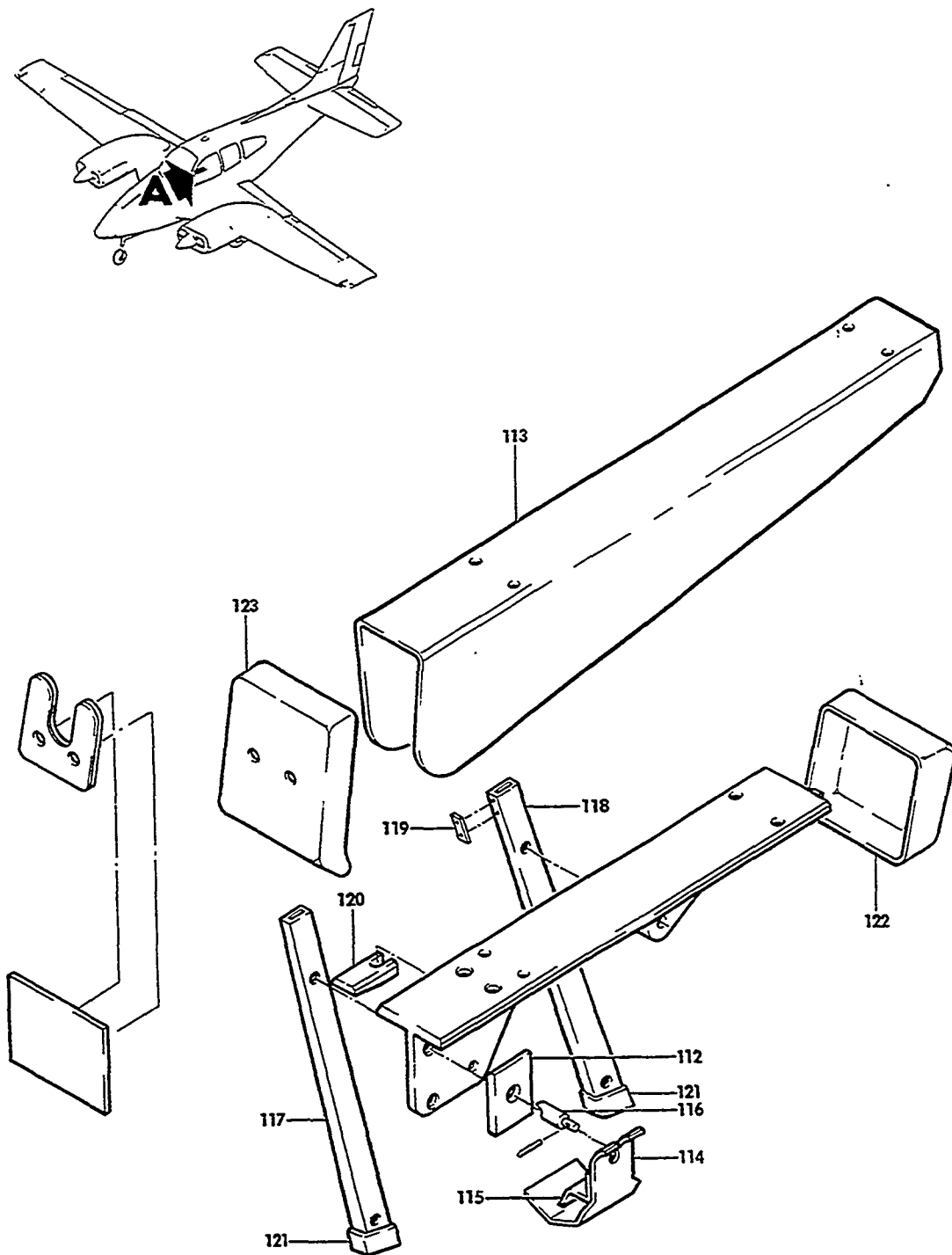
VIEW A
