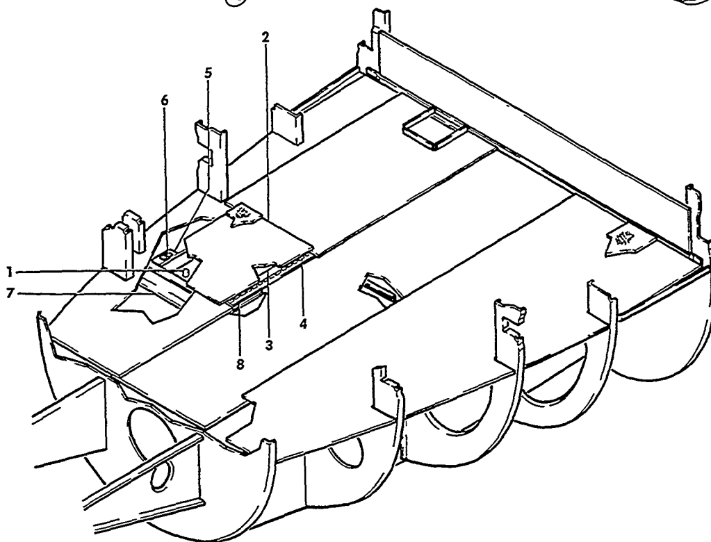
VIEW A
