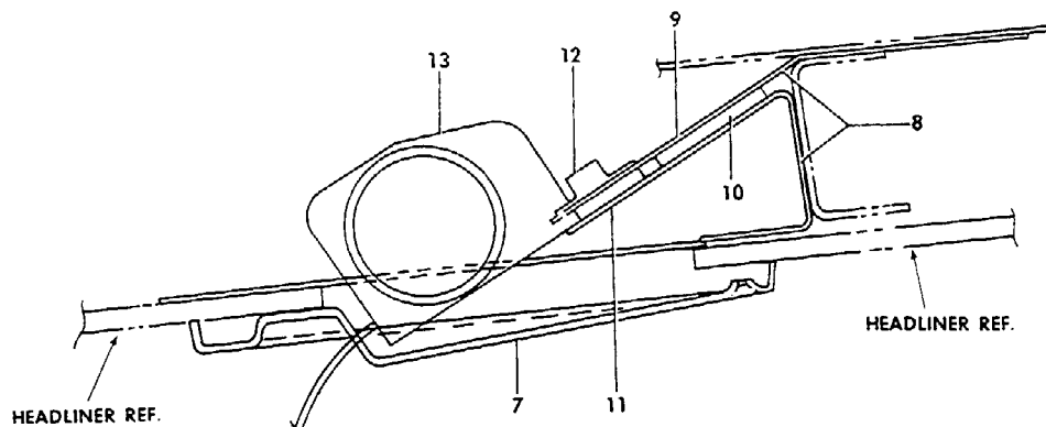
VIEW A
