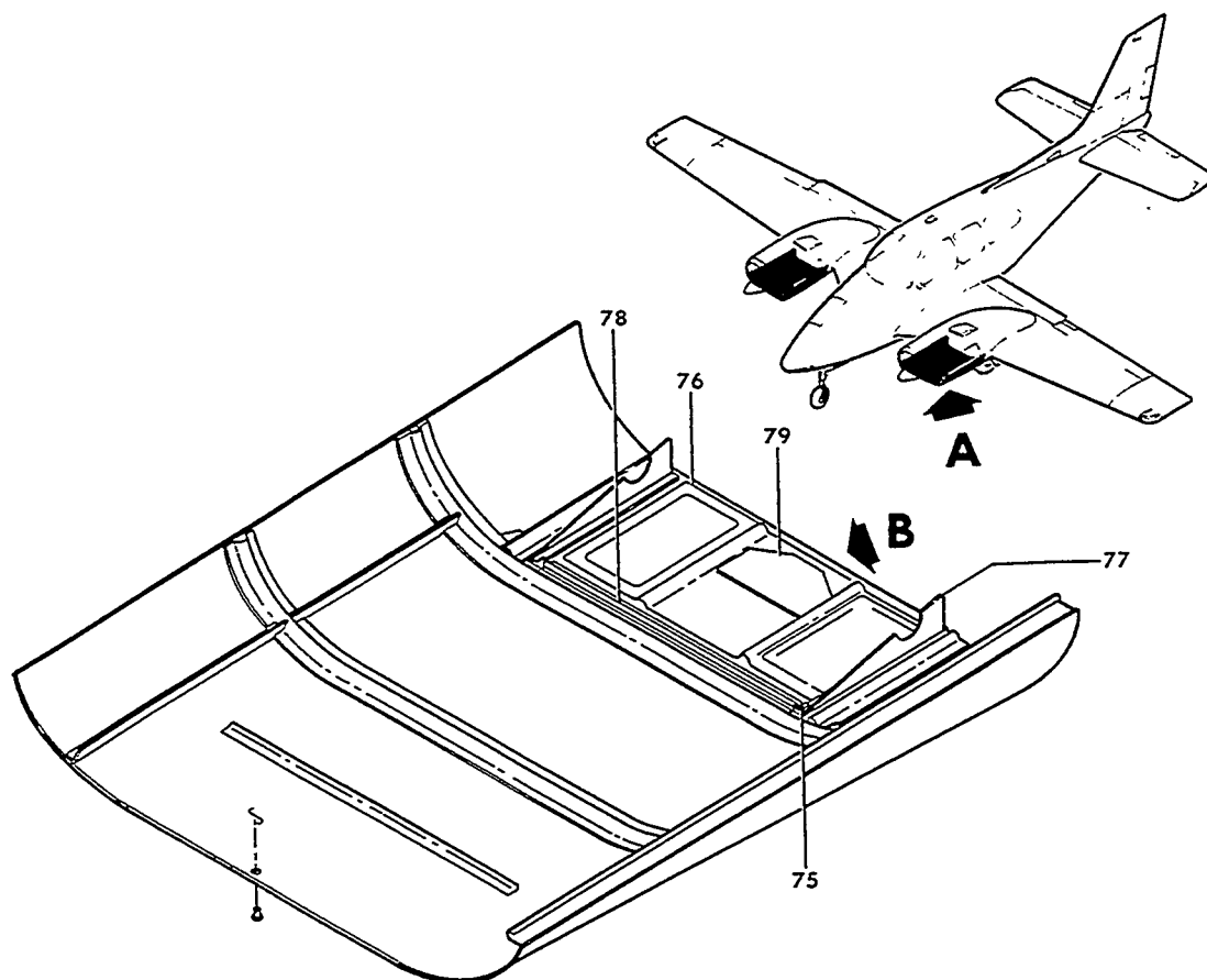
VIEW A
