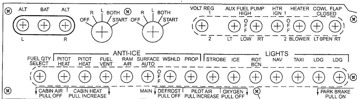
VIEW B
