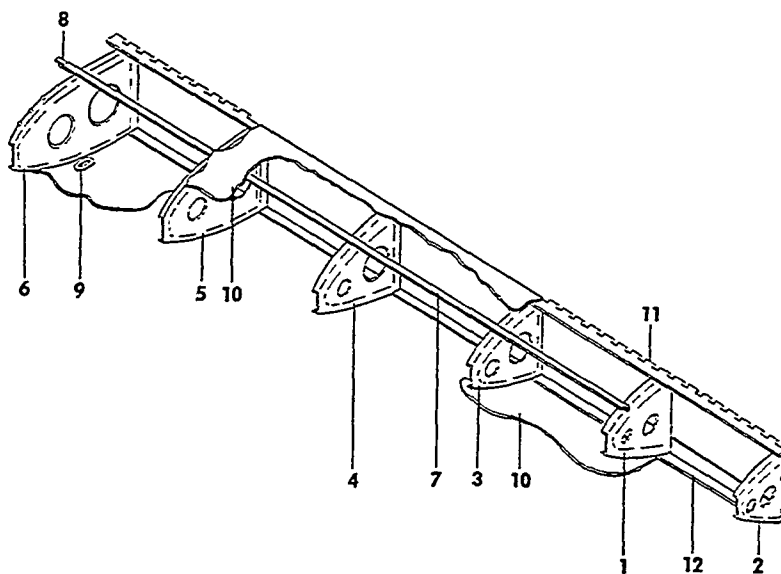
VIEW A
