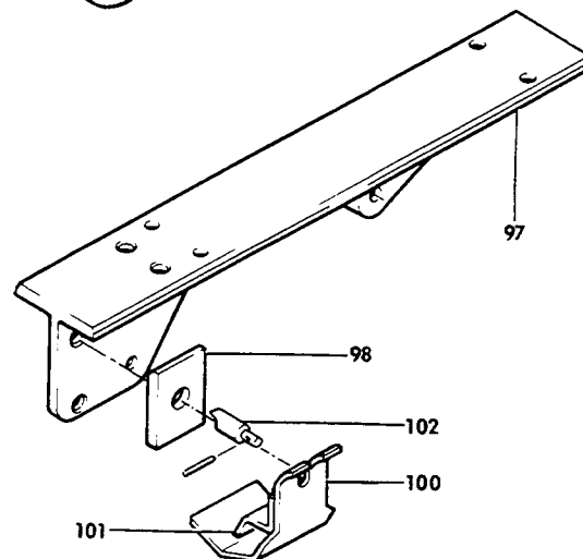
VIEW A
