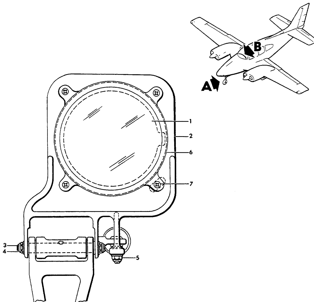
VIEW A
