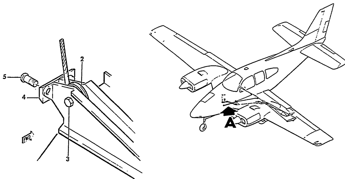
VIEW B
