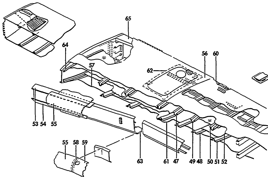
VIEW A
