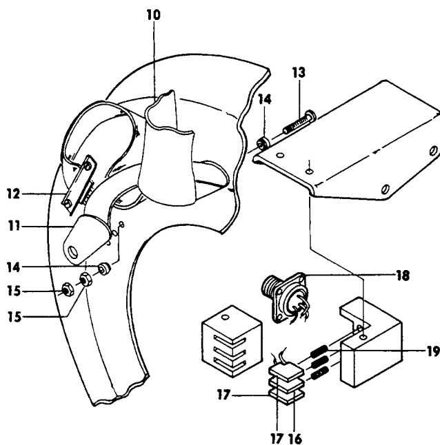
VIEW A
