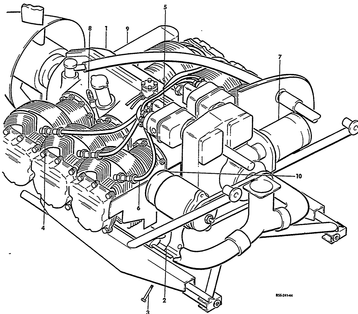
VIEW A
