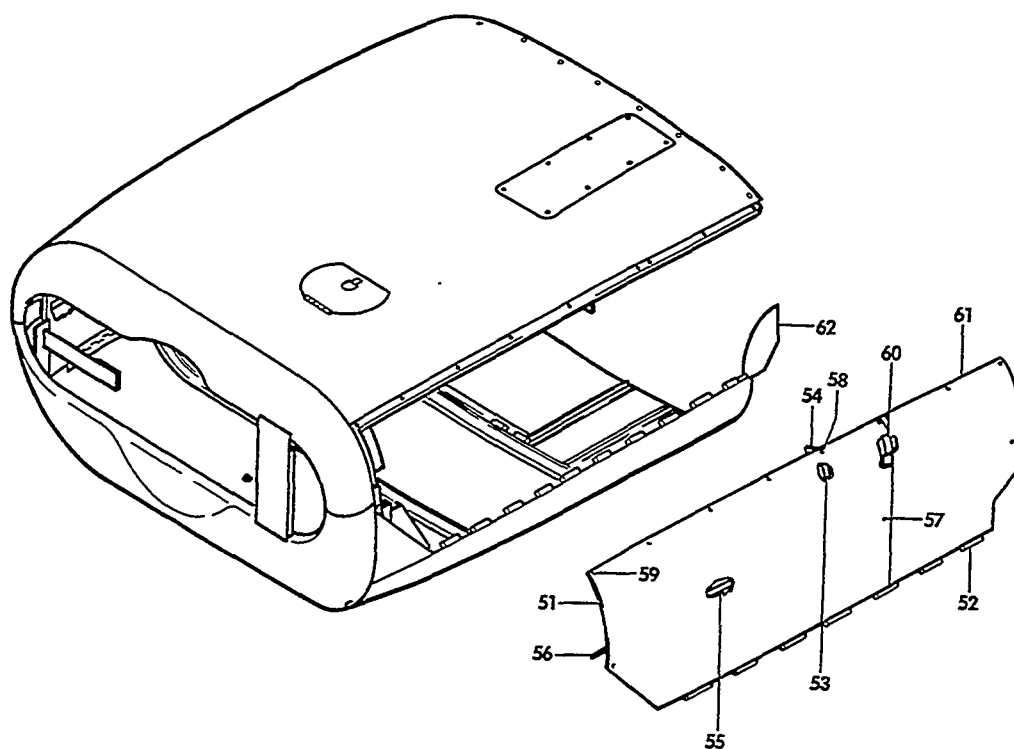
VIEW A
