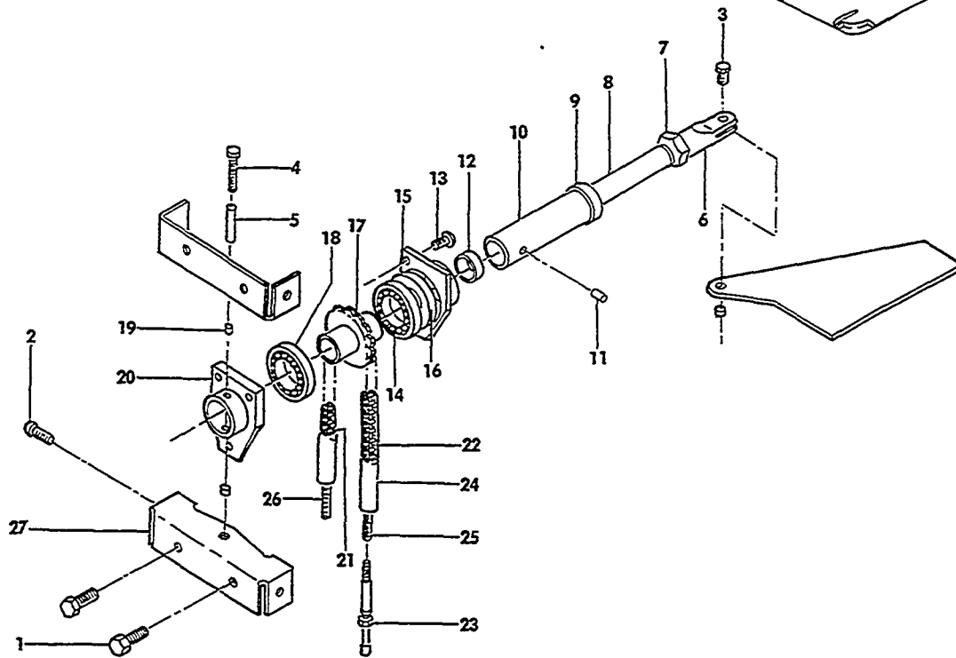
VIEW A
