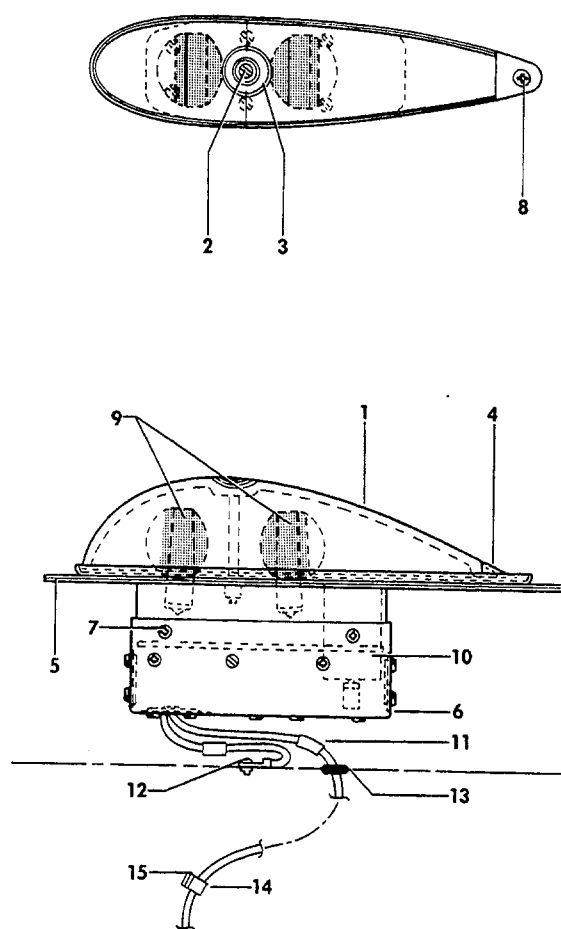
BEACON ASSY UPPER OSCILLATING
