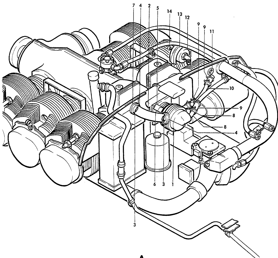
VIEW A
