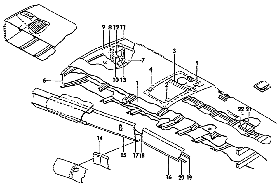
VIEW A
