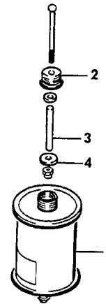
VIEW B
