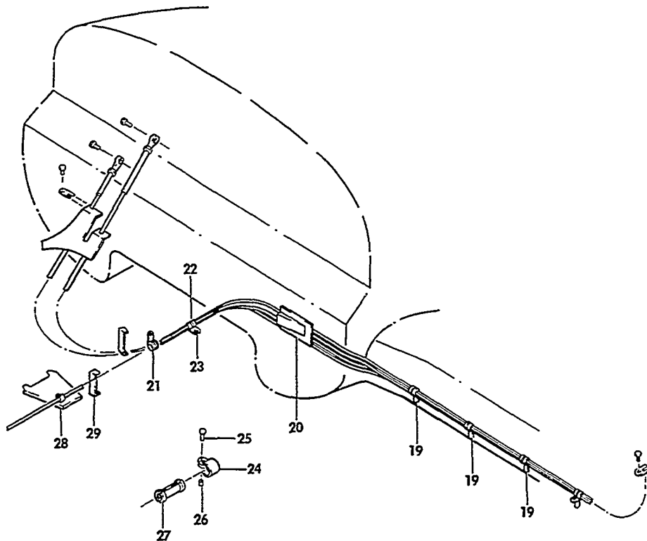
VIEW A
