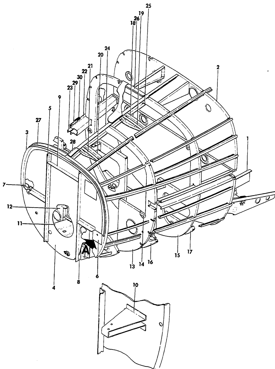
VIEW A
