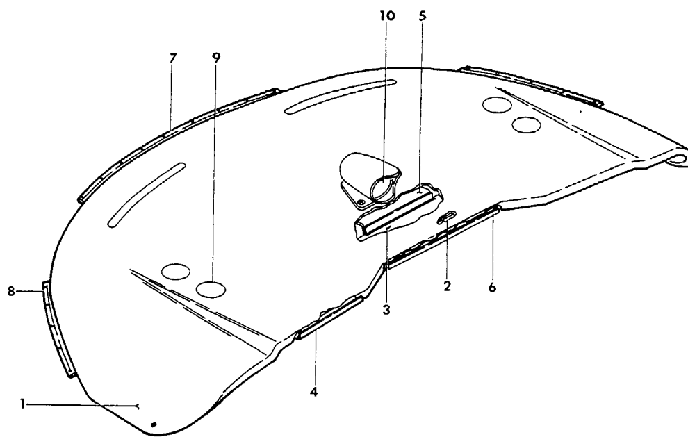
VIEW A
