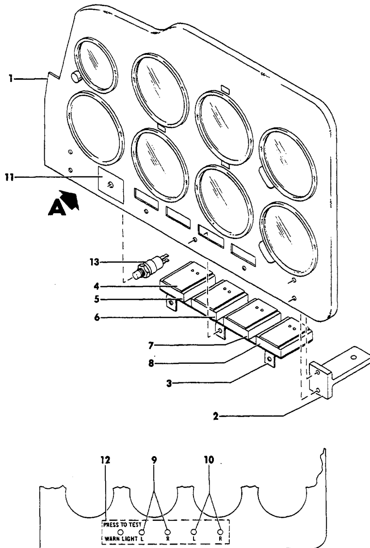
VIEW A
