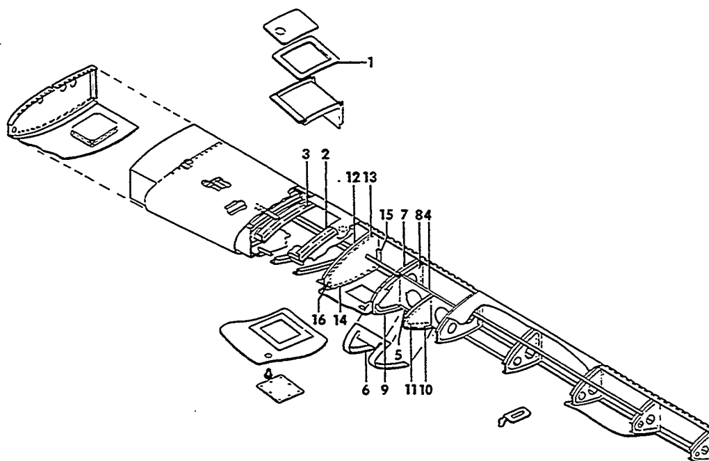
VIEW A
